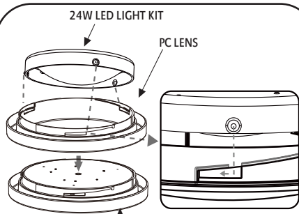
Fig. 19-1 24W LED ASSEMBLY
