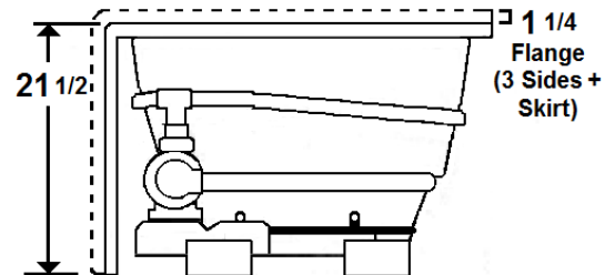
Standard (S) Pump, Blower, & Heater Location
