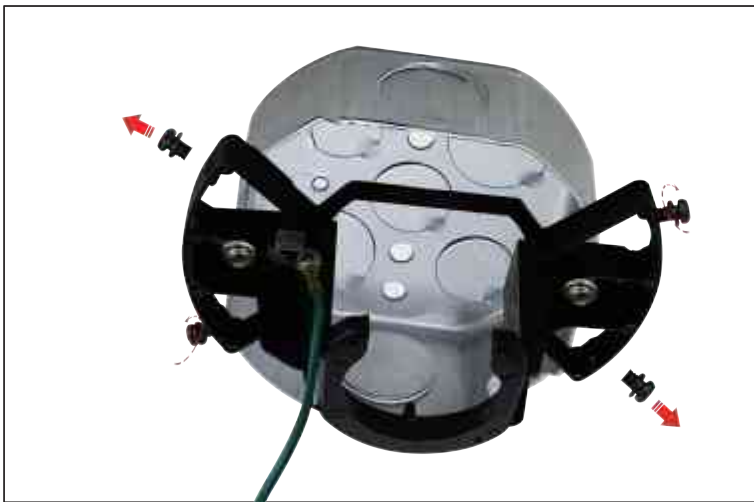
Step 7 Remove 2 opposite screws and loosn the other 2 screws.
