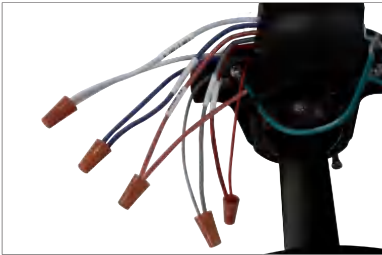
Step 9 Connect the same color wires from the fan and receiver.
