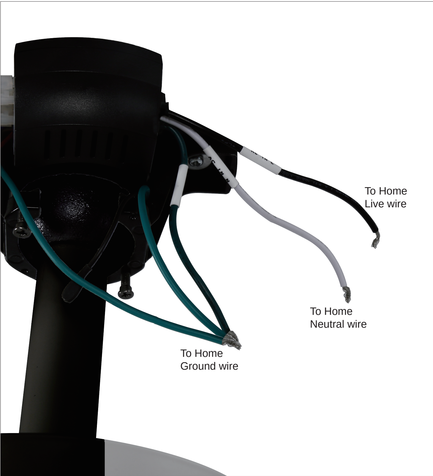
Step 10 Connect the receiver to home wires. Black for Live wire, White for neutral wire, Green for ground wire
