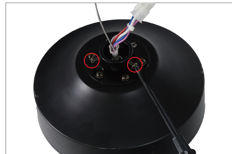
Step 2 Loosen two screws on the coupler.
