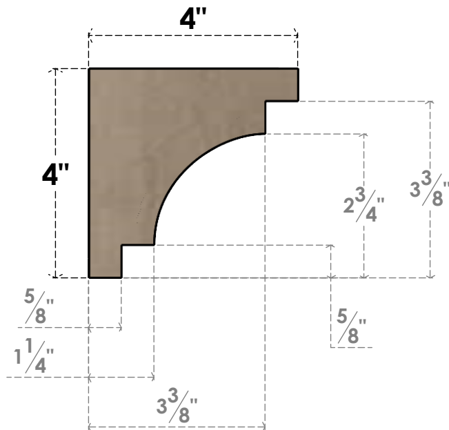
SIDE PROFILE
