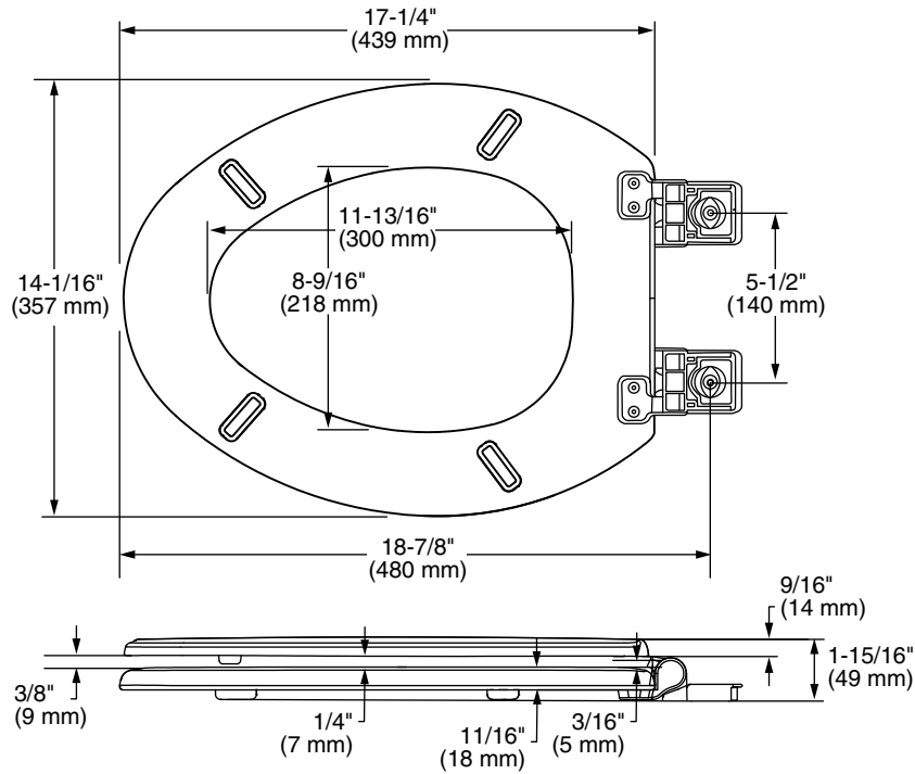
5269A.65DL Elongated Toilet Seat
