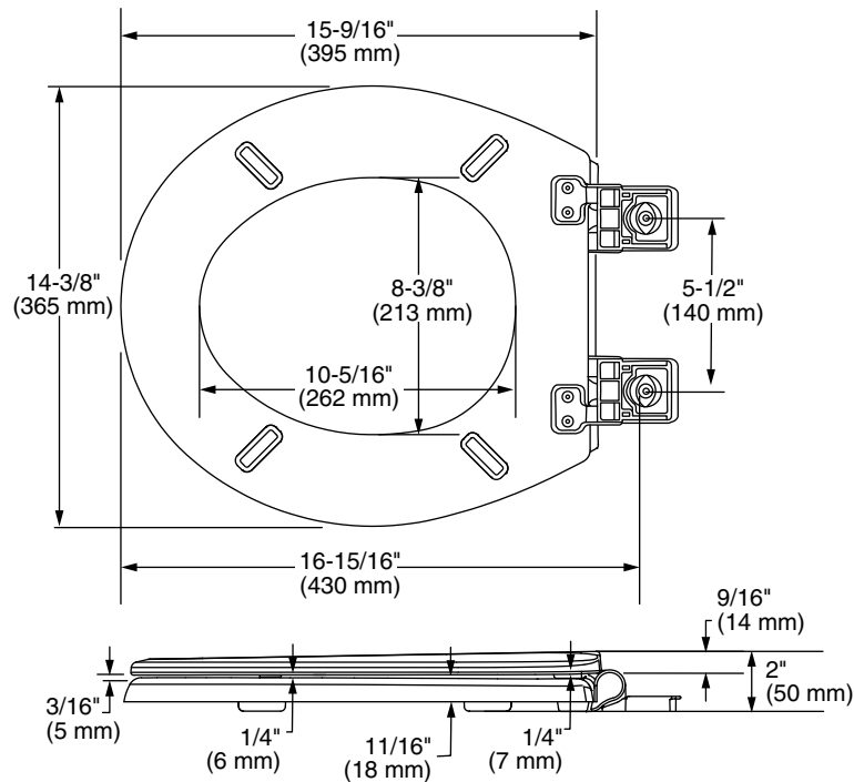
5269B.65DL Round Front Toilet Seat
