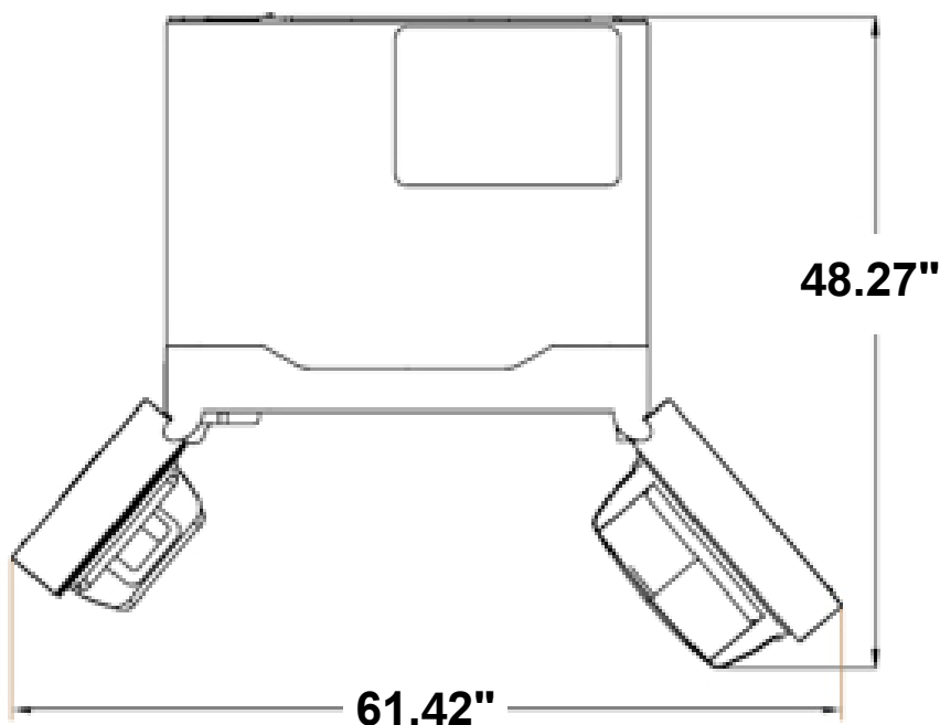
TOP VIEW, OPEN 135°
