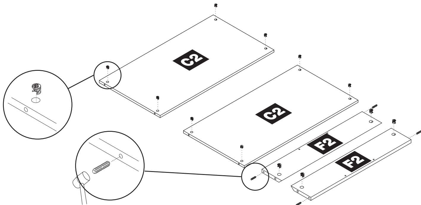
CAM LOCK (QTY. 12) CIERRE DE LEVA
