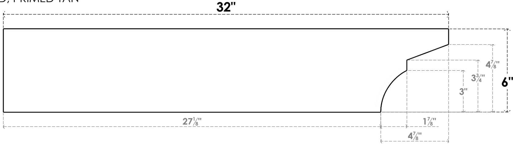
SIDE PROFILE
