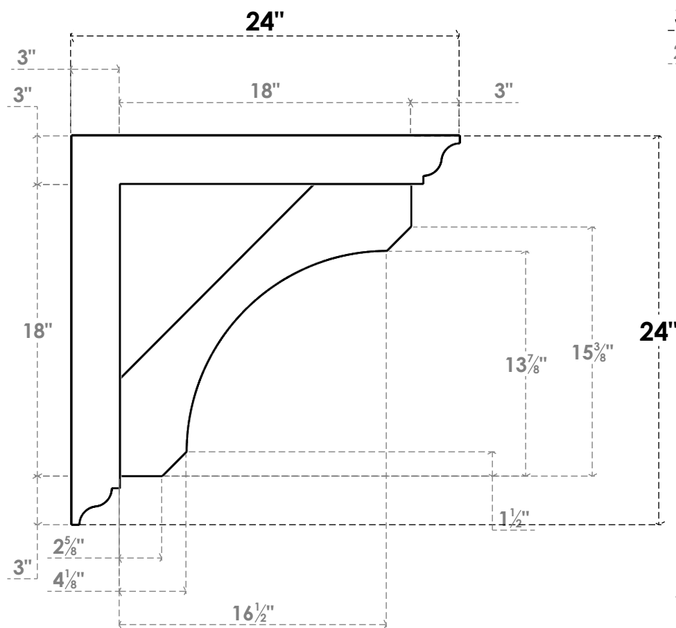
SIDE PROFILE
