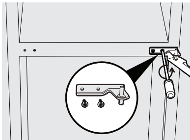
Extraiga la bisagra central
