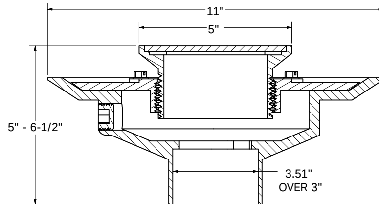
SECTION A-A SCALE .65
