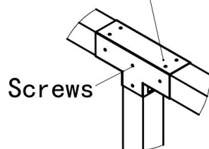
Pergola Bracket
