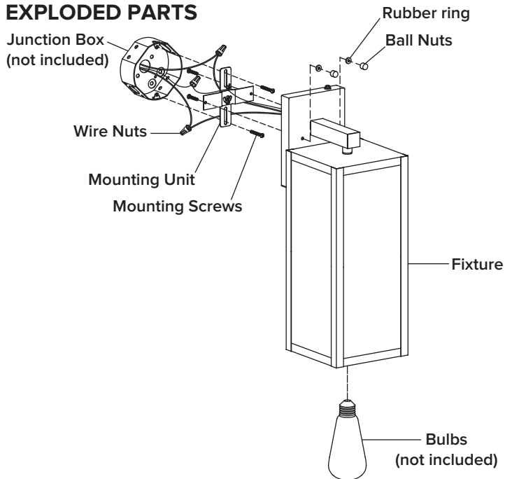
Mounting Unit
