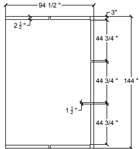
PLAN A LA BASE PLAN AT THE BASE
