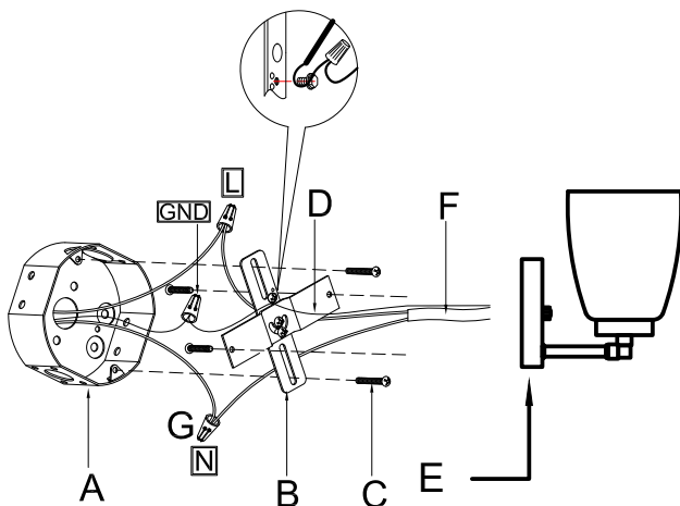
Wire Connection Diagram:
