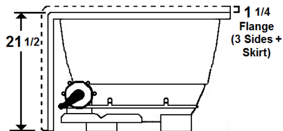
Standard (S) Blower Location
