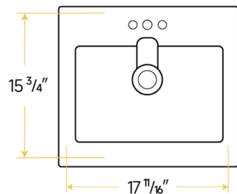
Cutout Size
