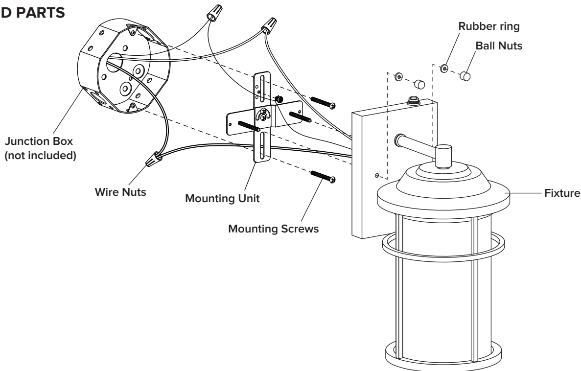
Mounting Unit
