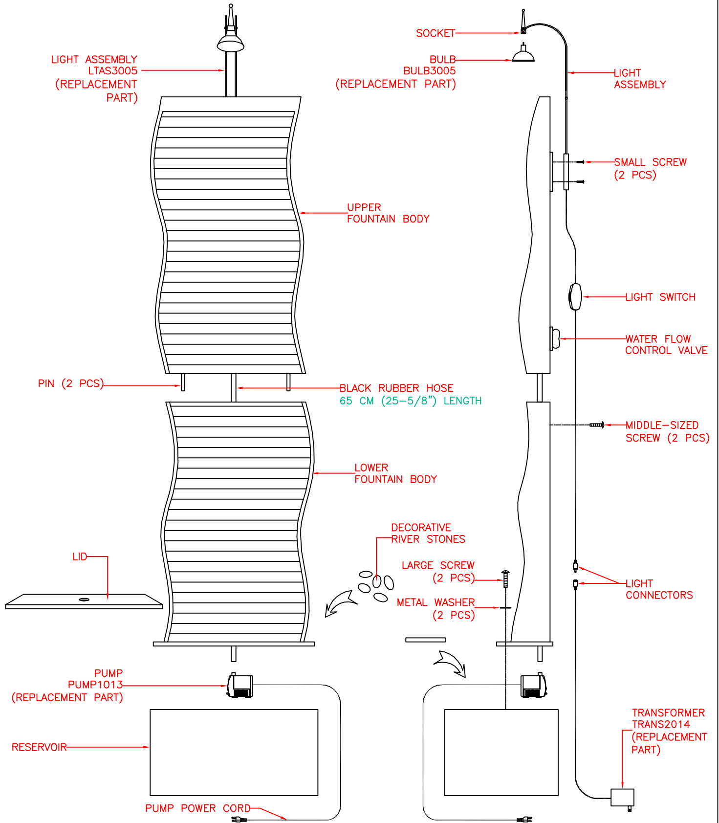
FRONT VIEW:
