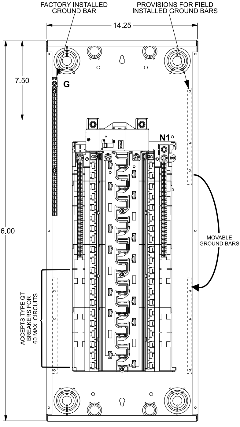
VIEW SHOWN WITH TRIM ASSEMBLY REMOVED
