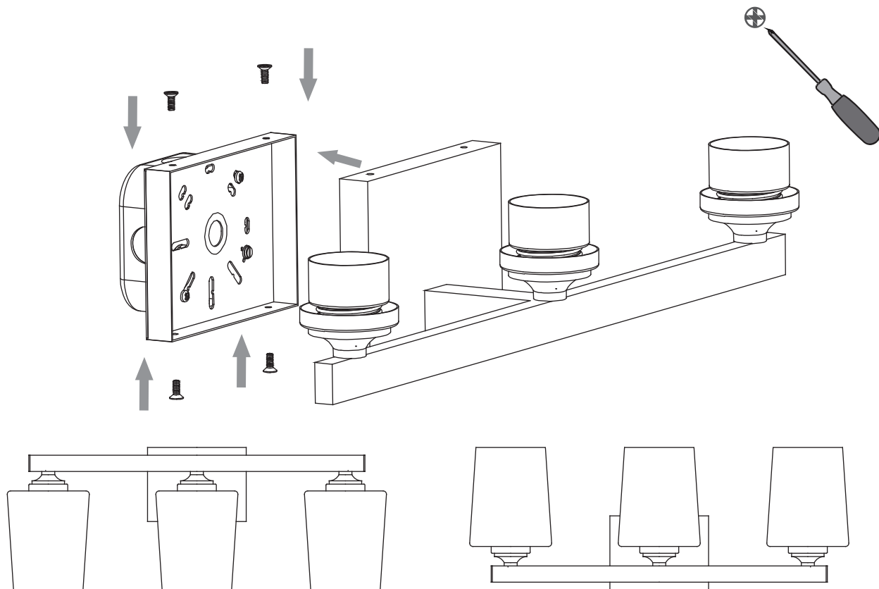
Installation Option 1: Down light
