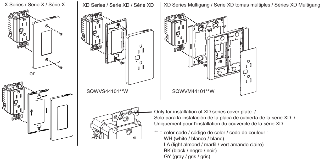
Figure / Figura / Figure 2 : Wall Plates / Placas de pared / Plaque murales
