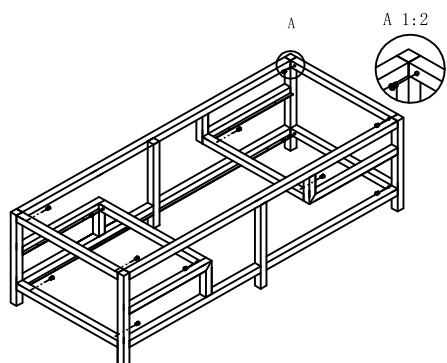
Frame Installation
