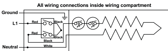
Figure 3 Wiring Diagram for use with 120 volt heater
