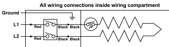
Figure 2 Wiring Diagram for use with 240 and 208 volt heater
