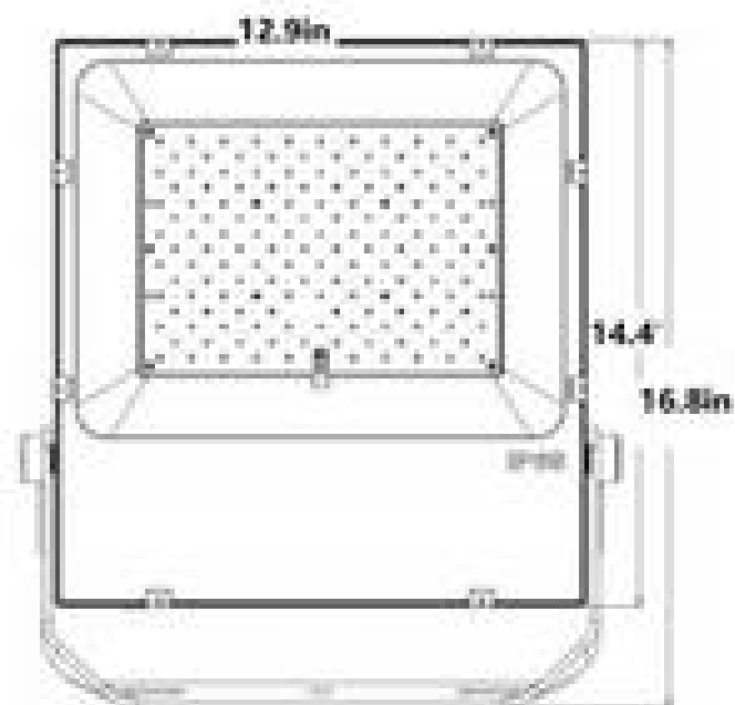
150W
