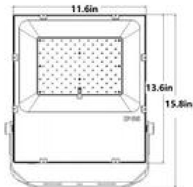
80W-100W
