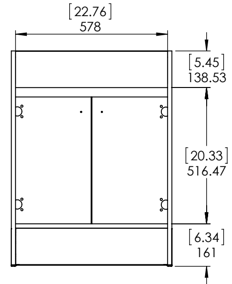
BACK VIEW
