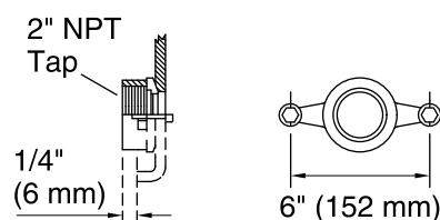
Outlet Detail
