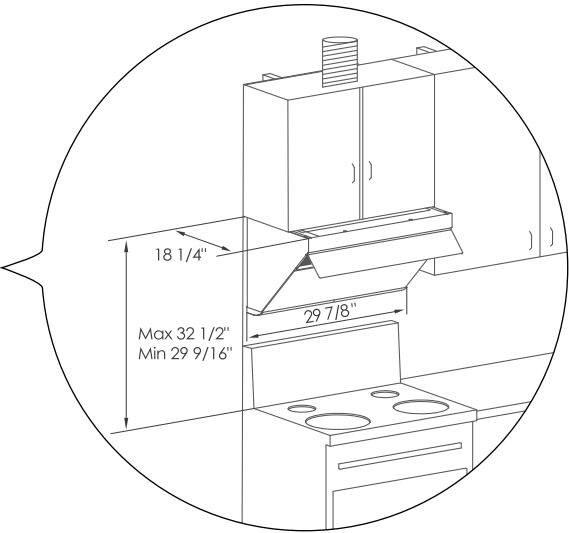
Under-Cabinet Installation
