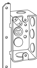
58371-T-1/2 "T" bracket recessed 1/2"
