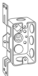
58361-V-1/2 "CV" bracket recessed 1/2"
