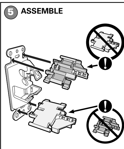
Snap the lock tabs in place.
