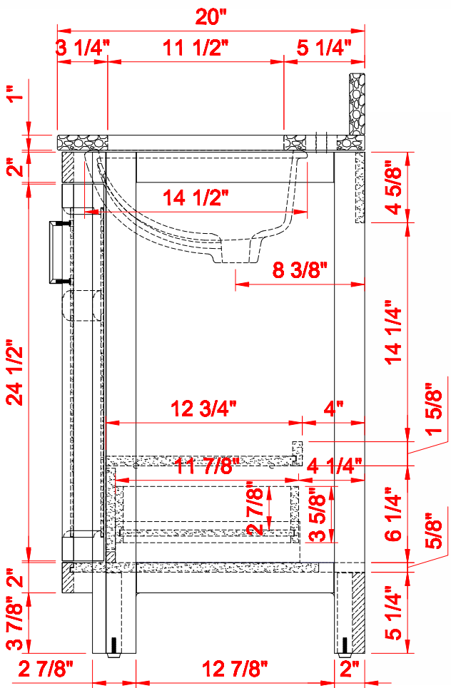
SIDE VIEW
