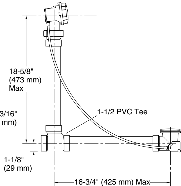
Above-the-Floor
