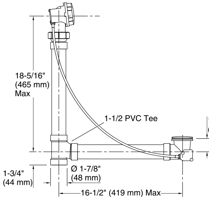
Through-the-Floor
