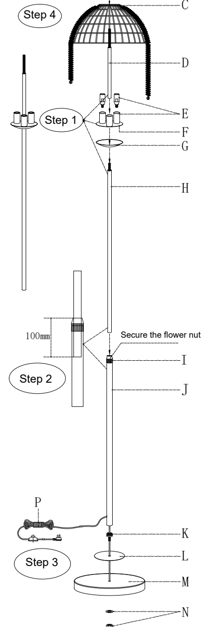
L6203/400 Floor lamp
