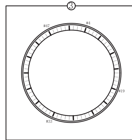
Complete installation drawing of spring
