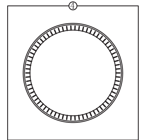
Complete installation drawing of spring
