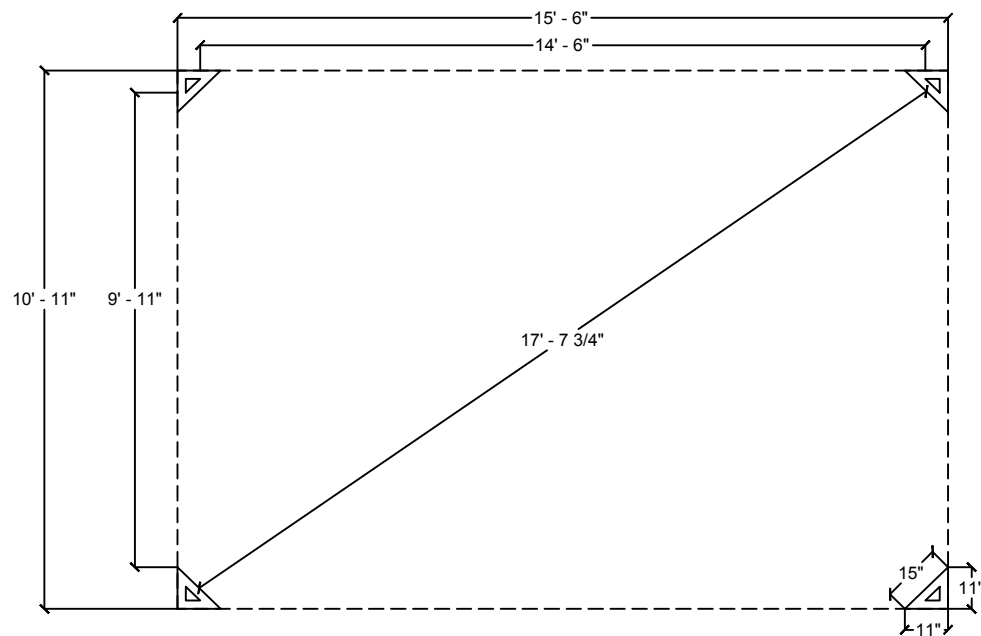
PLAN A LA BASE DES PATTES PLAN AT THE BASE OF THE LEGS
