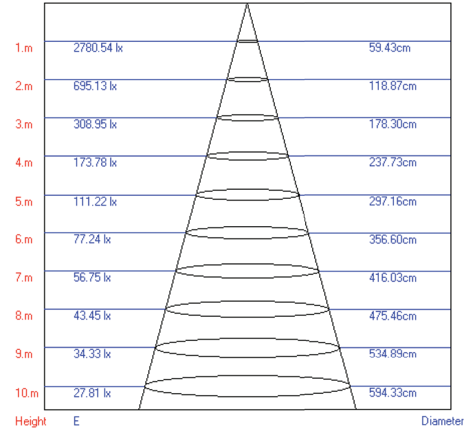
Lux-Distance Curve
