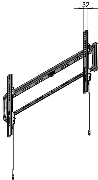
ORTHOGRAPHIC VIEW
