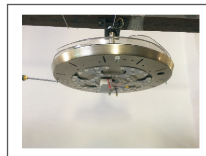
Step 4. Remove the screws on the side of the main engine chassis mounting attachment.
