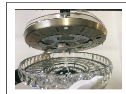
Step 5. Connect the Bluetooth drive cable on the lampshade with the Bluetooth cable on the chassis of the fan lamp host.
