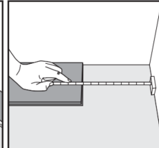
Fig. 5 At the end of the first row, put a 3/8" spacer along the wall, measure the length of the last plank to fit.
