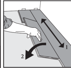
Fig. 10 Hint for installing planks. The long sides of planks must be fully aligned before rotating down. You cannot force the boards. If they are not lying flat, the long side is not fully engaged. Start over ensuring the long sides are fully engaged.
