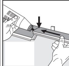
Fig. 2 Glue all of the short end joints in the first and last rows only. Use wood glue and weight down until glue has dried.
