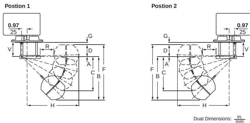
Figure 23: Travel Dimensions
