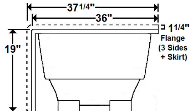
Standard (S) Pump Location
