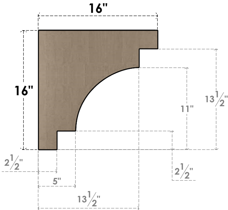
SIDE PROFILE
