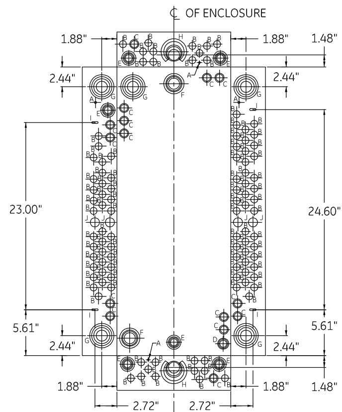
KNOCKOUT DIAGRAM
