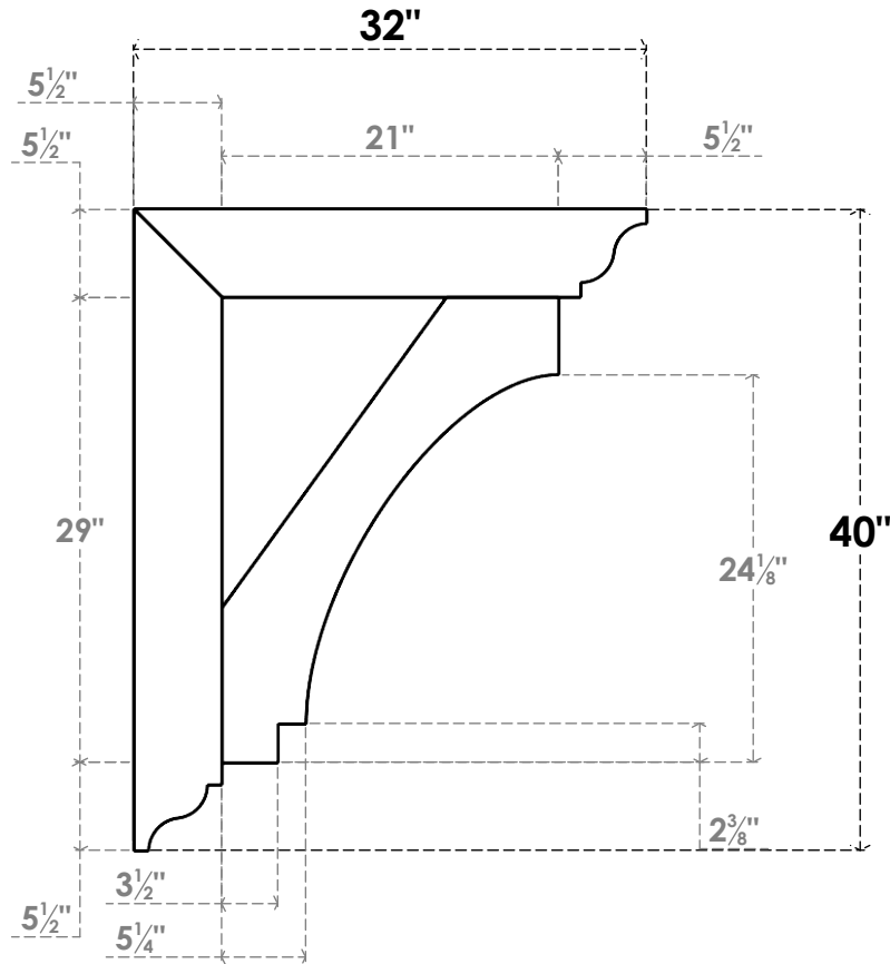
SIDE PROFILE
