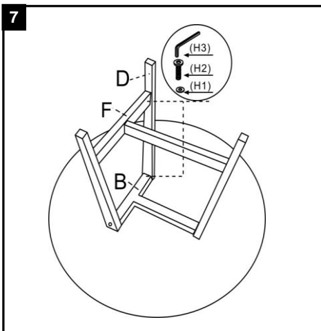
Step 7 Attach D to F & B, using allen bolt and washer (H1 & H2), tighten with allen key (H3)
