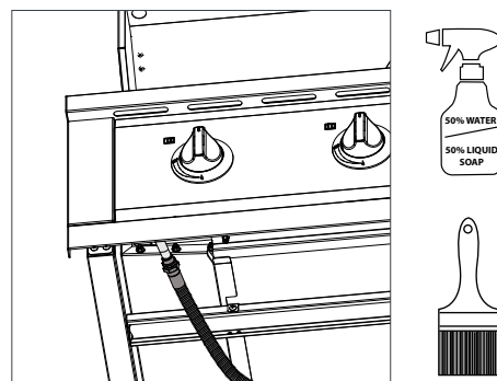
Leak Testing Diagram
