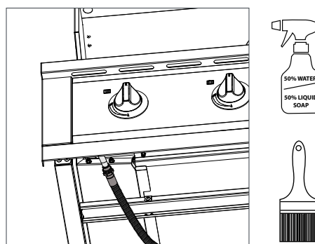
Leak Testing Diagram
