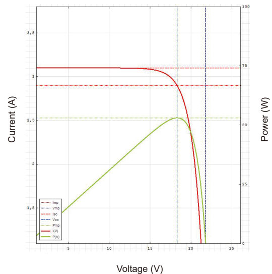
RNG-50D-SS Characteristics Versus Voltage
