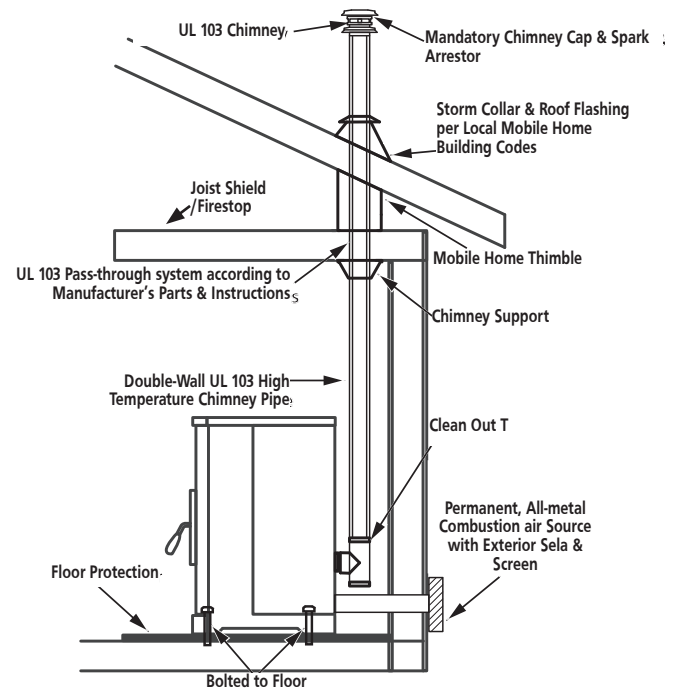
Figure 12: Mobile Home Vertical Chimney
