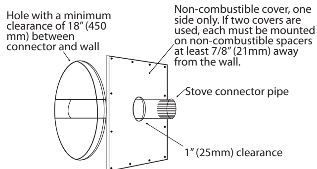
Figure 7: ONLY APPROVED CANADIAN WALL PASS THROUGH
