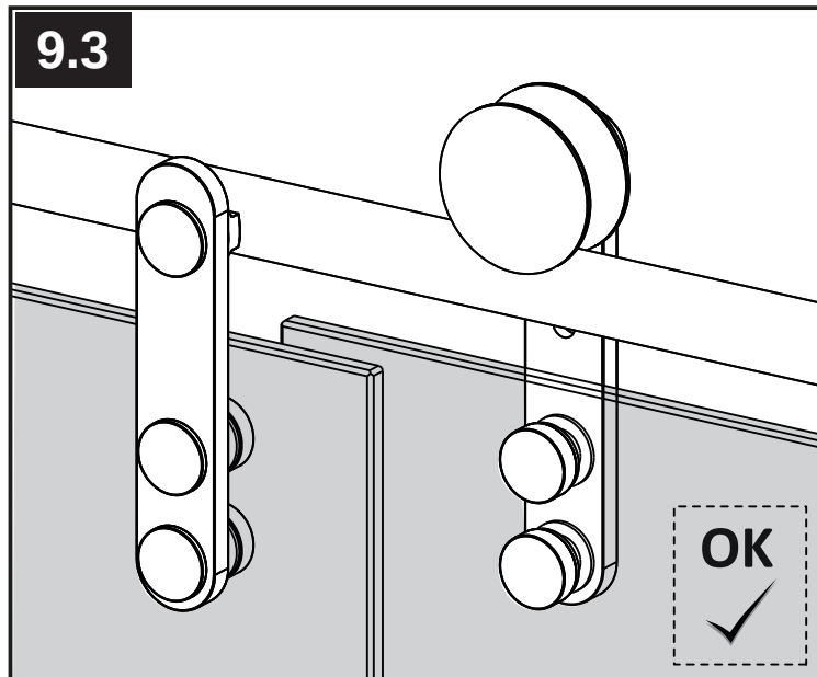
Sliding Glass Panel (G)
