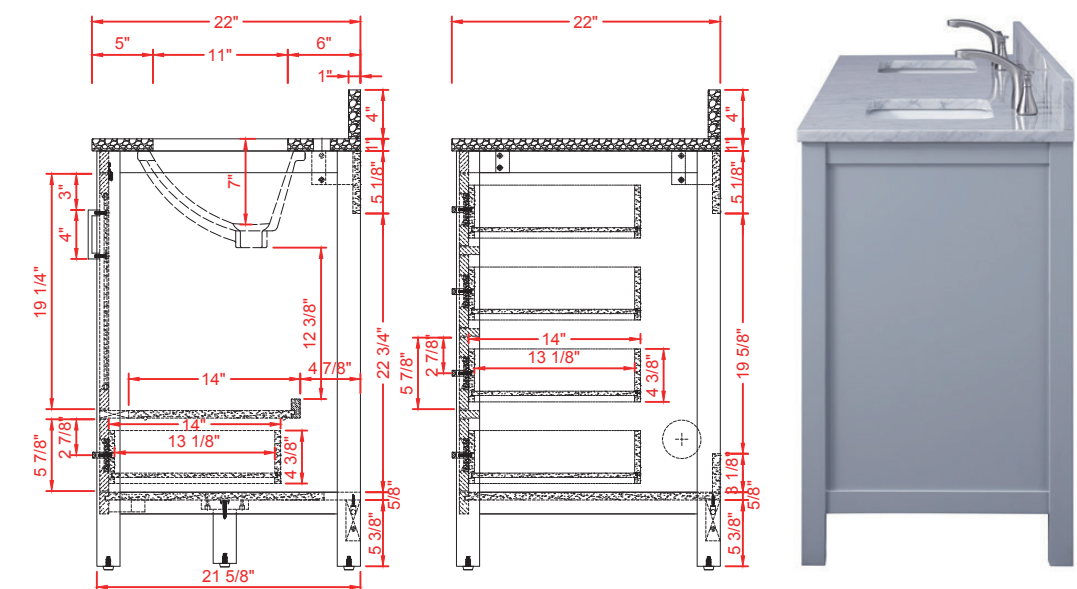
SIDE VIEW
