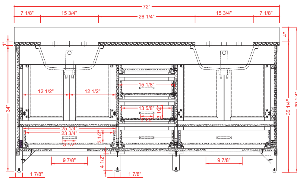
BACK VIEW
